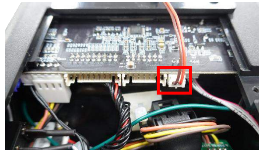
RTC connector
