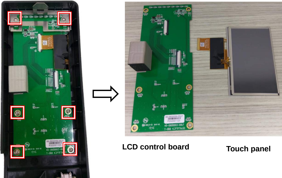
Screws location
