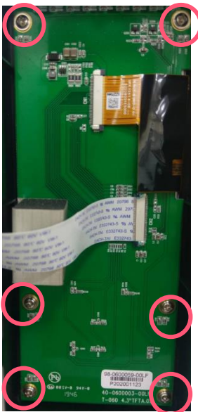
Screws location
